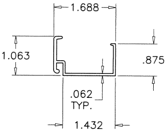
GLAZING BEAD (TRANSOM)
