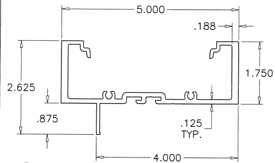
TRANSOM HEAD/SILL
