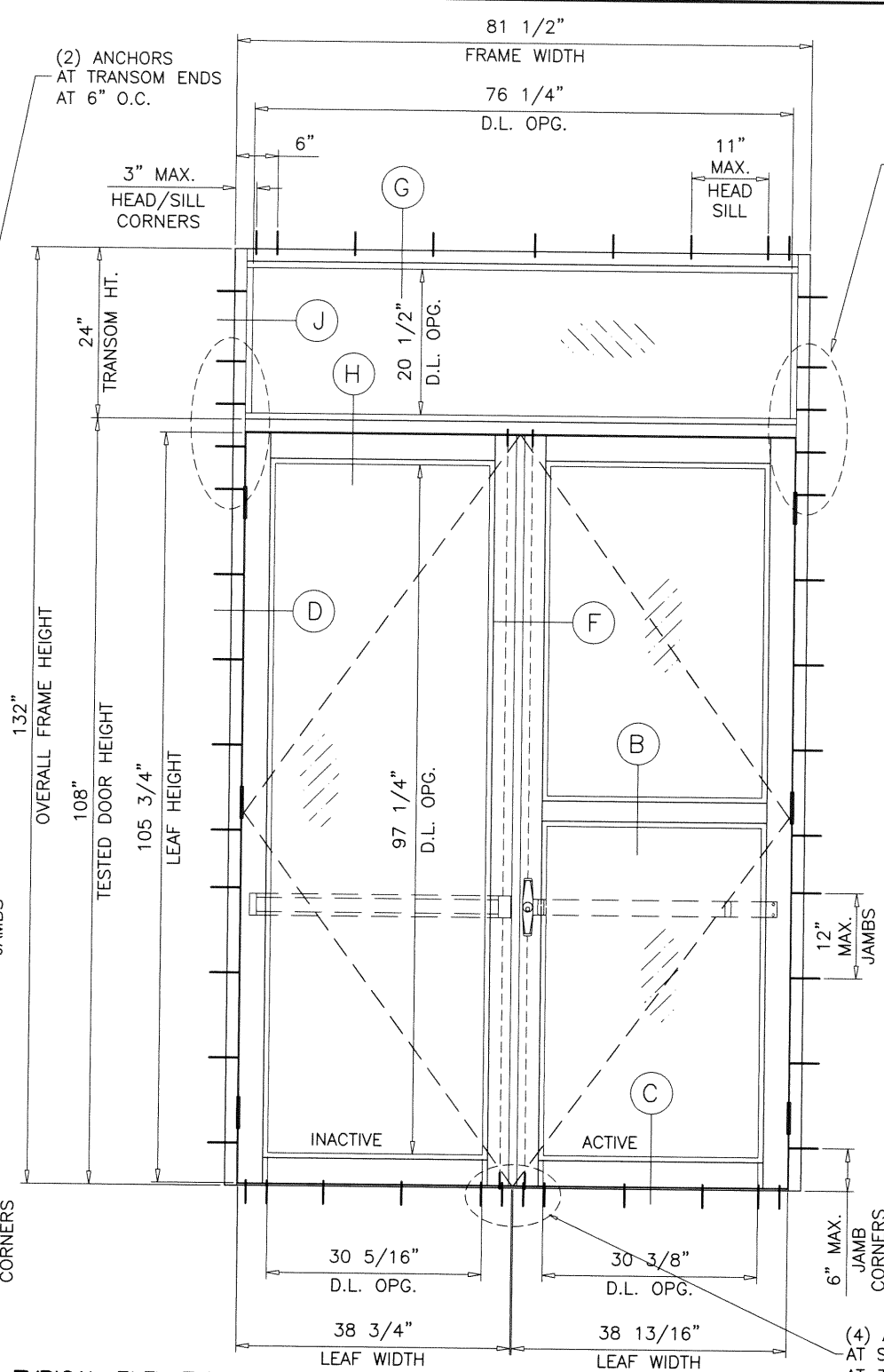
TYPICAL ELEVATION
