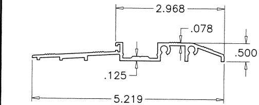
3 ADA THRESHOLD
