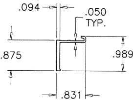
FRAME INSERT (TRANSOM)
