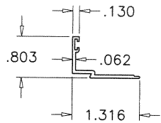
9 GLAZING BEAD INSUL. LAM. GLASS
